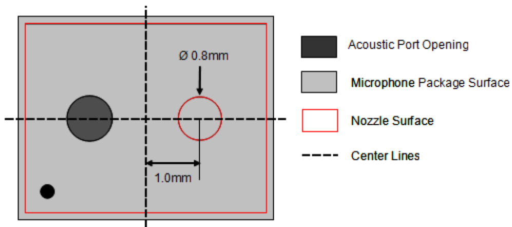
Figure 9: Recommended vacuum nozzle design.
